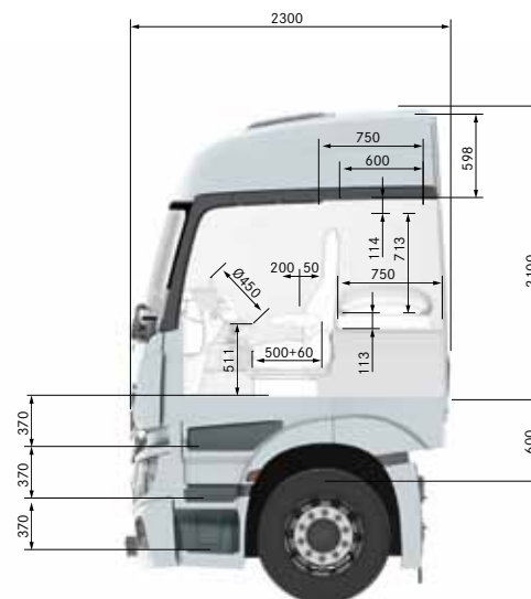
StreamSpace L-cab (3) (exterior width 2300 mm, engine tunnel)
